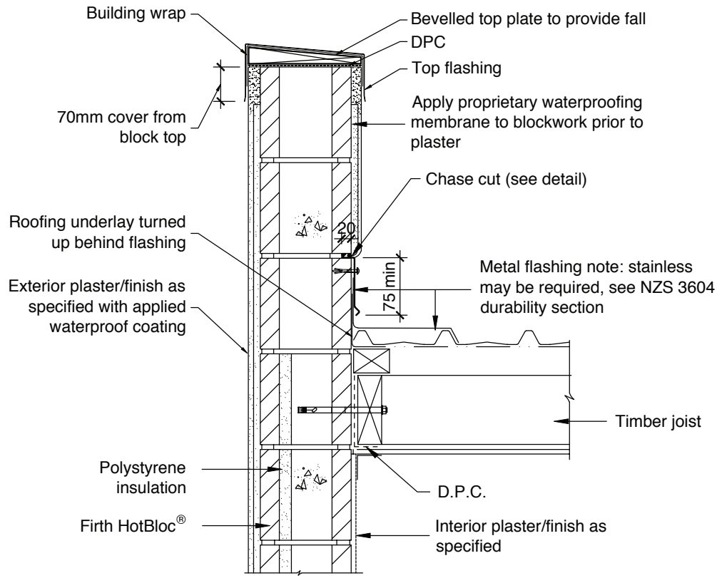
Parapet Wall Detail
