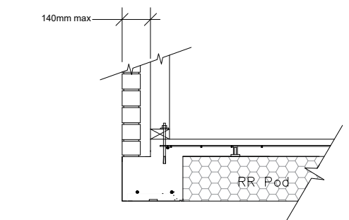
⑫ 220mm FIRTH RIBRAFT POLYPOD BRICK VENEER FIRTH RAFTMIX 20 OR 25MPa
