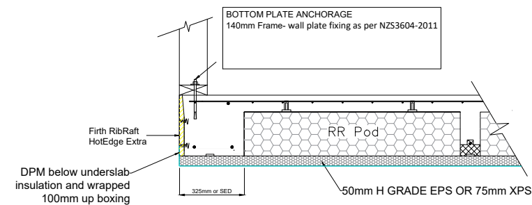
⑦ 220mm FIRTH RIBRAFT POLYPOD 140mm WALL FRAME HOTEDGE EXTRA & UNDERSLAB INSULATION FIRTH RAFTMIX 20 OR 25MPa
