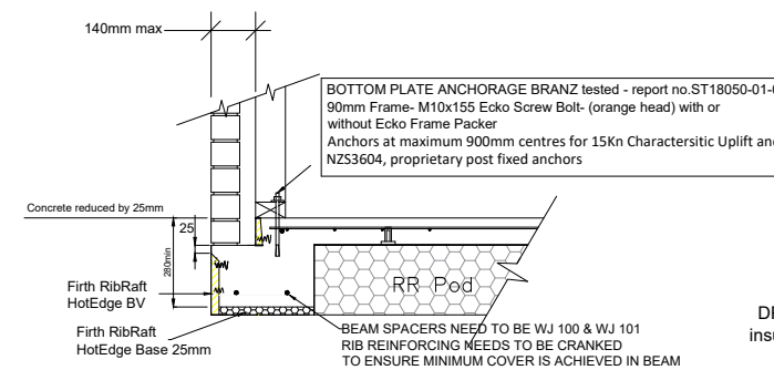
⑩ 220mm FIRTH RIBRAFT POLYPOD BRICK VENEER HOTEDGE & HOTEDGE BASE FIRTH RAFTMIX 20 OR 25MPa
