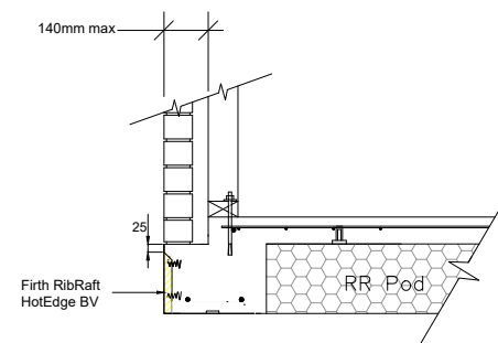
⑨ 220mm FIRTH RIBRAFT POLYPOD BRICK VENEER HOTEDGE FIRTH RAFTMIX 20 OR 25MPa
